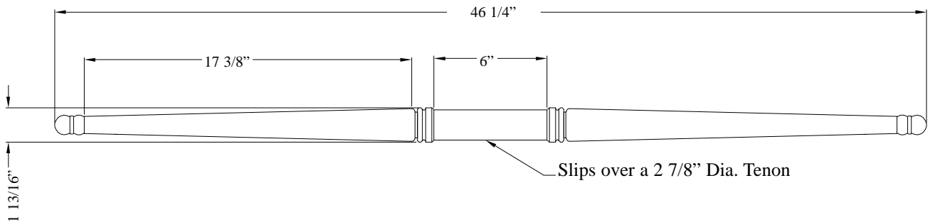
1 AARHNC-46-LR 1 Cast Aluminum Arm Hancock - 46 1/4" Ladder Rest
