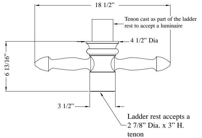
1 AARNBP-18-LR 1 Cast Aluminum Arm Newburyport - 18 1/2" - Ladder Rest
