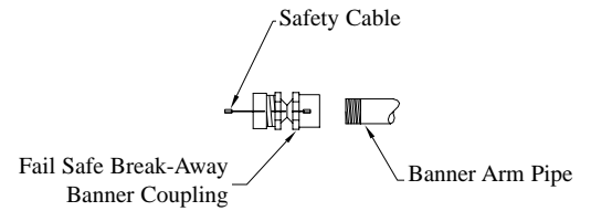
Detail of Breakaway Coupling
