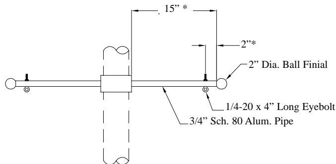
2 AARBK15-SC8-EB-FO2 2 Aluminum Arm Bracket 15" Arm Length - Schedule 80 Pipe- Eyebolt - 2" Ball Finial
