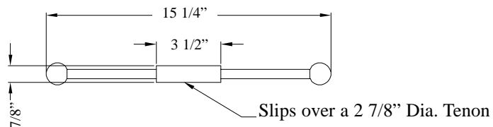
1 AARHRV-15-LR 1 Cast Aluminum Arm Harvard - 15 1/4" - Ladder Rest
