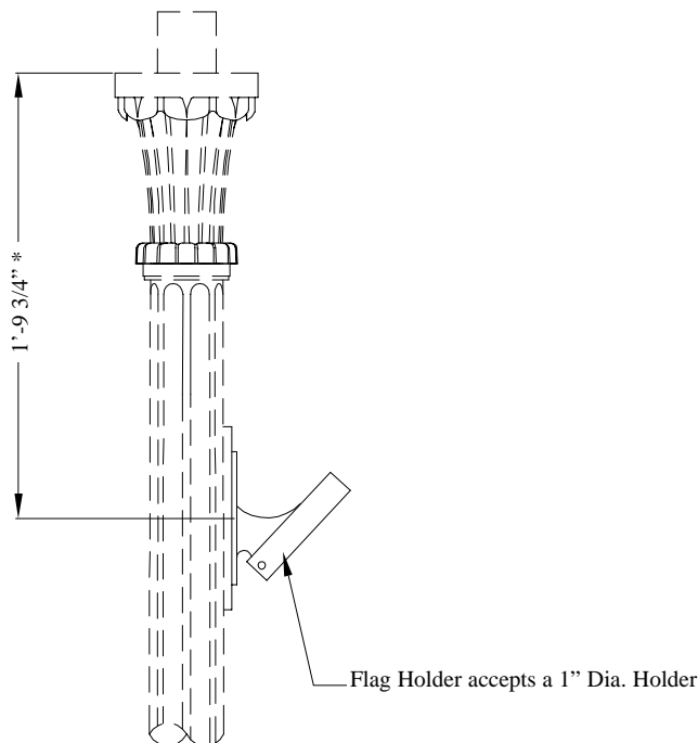
AARRDN-FH Aluminum Arm Radnor - Flag Holder
