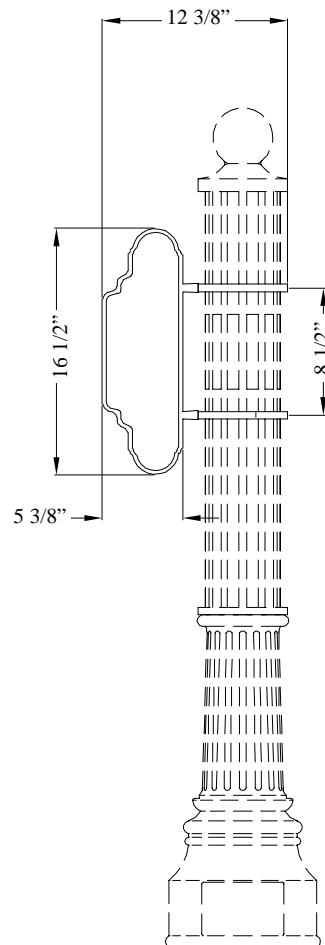
1 AARGTT - SS16.5 1 Cast Aluminum Arm Gettysburg - Street Sign 16.5"
