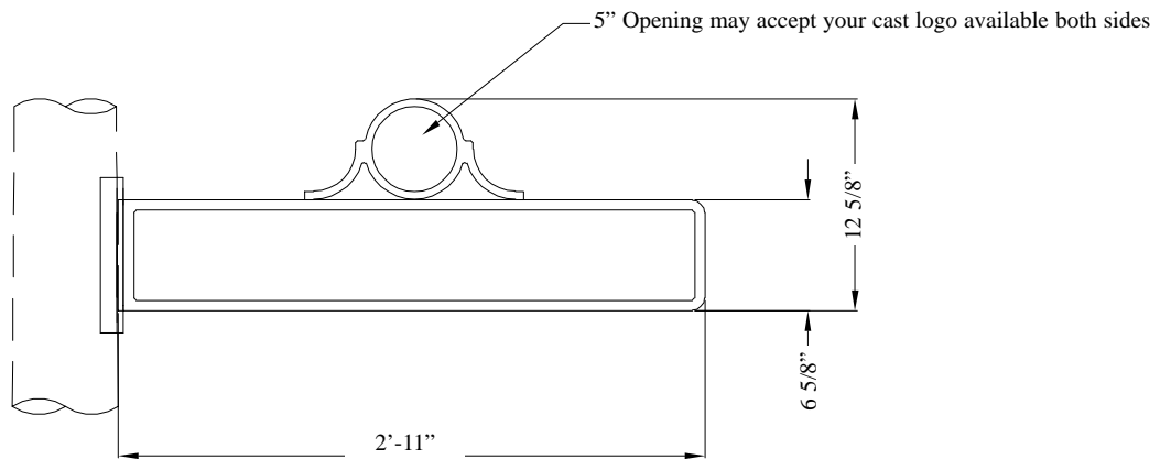
1 AARWTY-SS35 1 Aluminum Arm Westerly - Street Sign 35"
