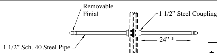
2 SARBN/CM24-SC4-WRC-RM 2 Steel Arms Banner Arms / Clamp on 24" Banner Width - Schedule 40 pipe - Worcester Finial - Removable
