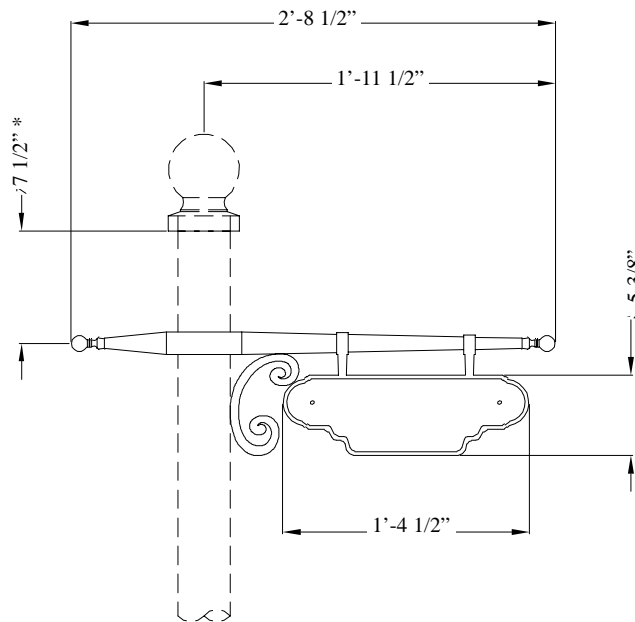
1 AARHRV- SS23 1 Cast Aluminum Arm Harvard - Street Sign 23"
