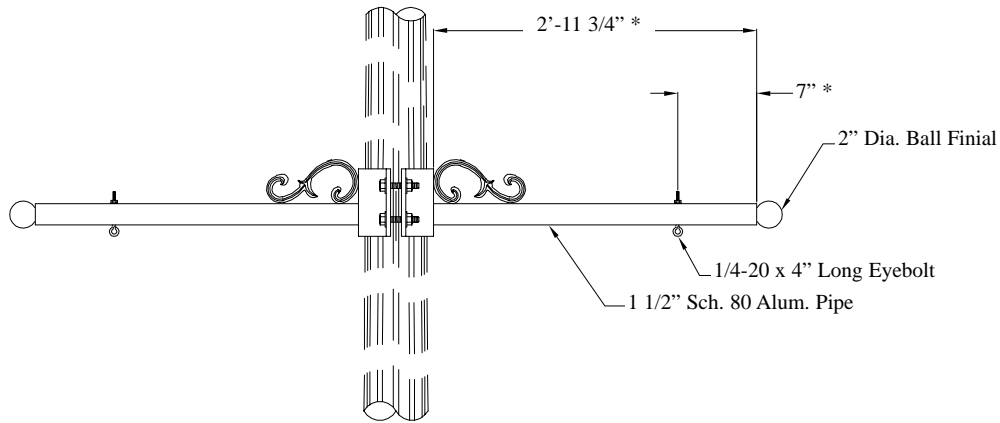
2 AARBK/CM35.75-SC8-EB-FO2 2 Aluminum Arm Bracket / Clamp Style 35 3/4" Arm Length-Schedule 80 Pipe - Eyebolt - 2" Ball Finial
