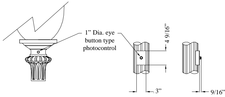
Post Mounted Button Type Photo Control.
