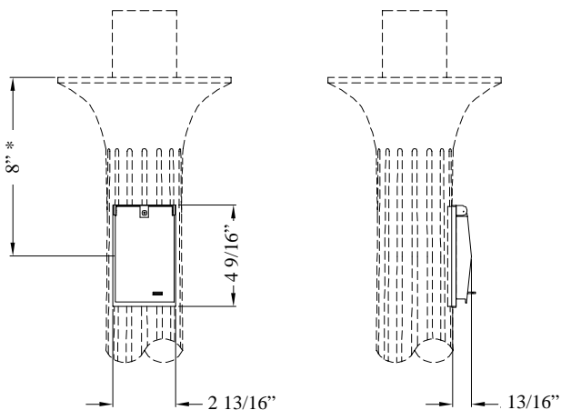
DX/WN-V1 Duplex Receptacle w/ Standard Weatherproof Cover-120 Volt
