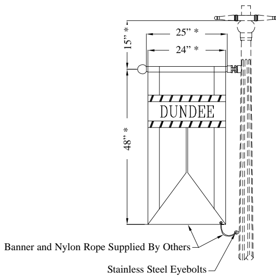
1 AARB/BA24-SC8-EB-FO2-RM 1 Aluminum Arm Banner Arm / Breakaway 24" Banner Width - Schedule 80 pipe - Eyebolt - 2" Ball finial - Removable
