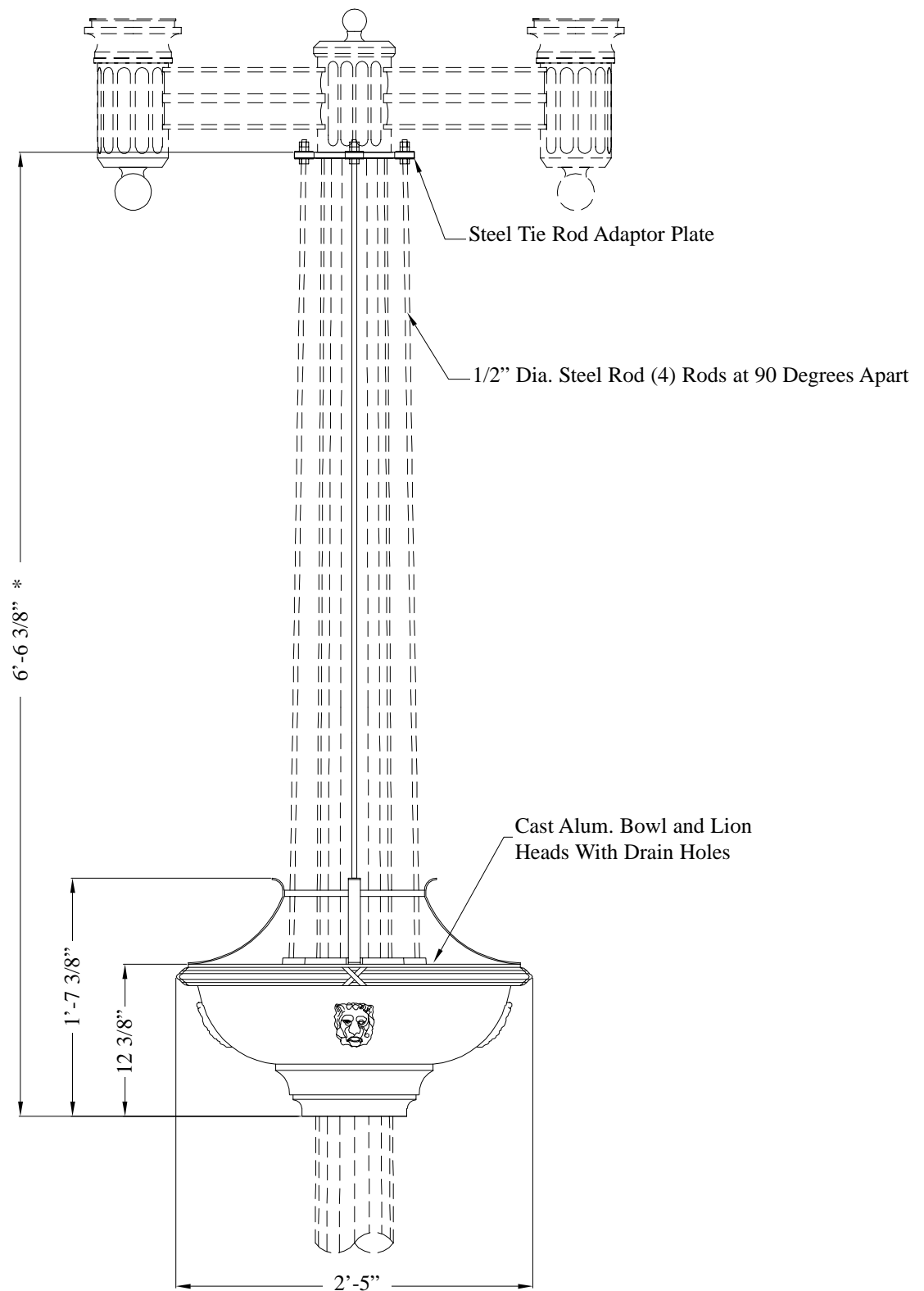
1 ABKALN 1 Aluminum Bracket Allentown Bowl Assembly
