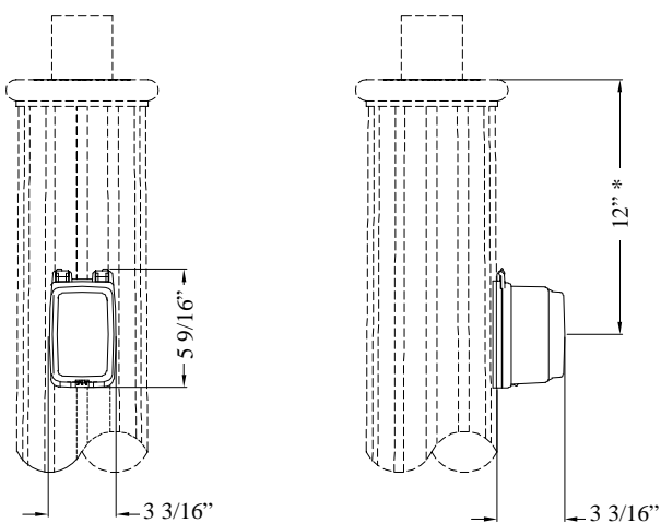
GF/WI-V1 GFI Receptacle w/ Weatherproof In Use Cover-120 Volt
