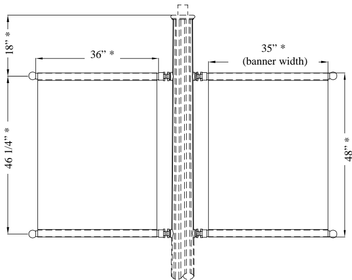
4 AARB/BA35-SC8-FO2-RM 4 Aluminum Arms Banner Arms / Breakaway 35" Banner Width- Schedule 80 pipe - 2" Ball finial - Removable
