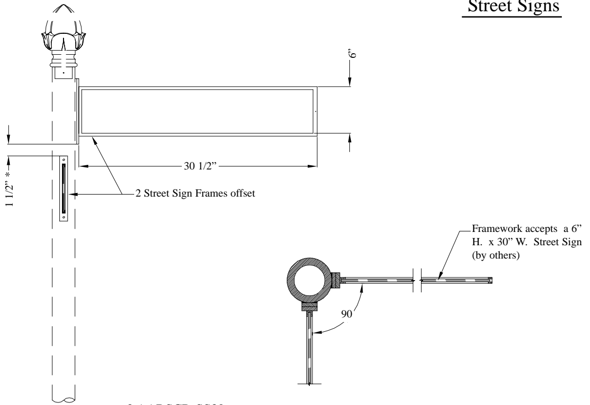
2 AARSCR-SS30 2 Aluminum Arms Scarsdale - Street Signs 30.5"
