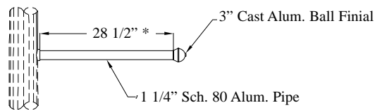
1AARB28.5-SC8-FO3-RM 1 Aluminum Arm Banner Arm 28" Banner Width - Schedule 80 pipe - 3" Ball Finial - Removable
