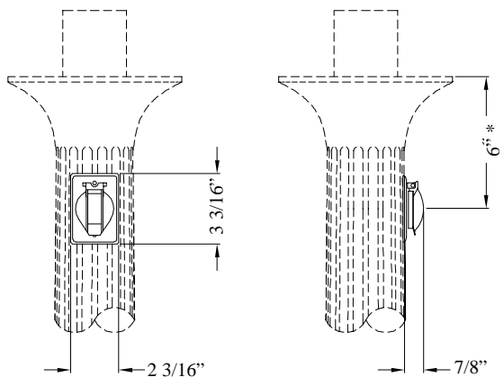
SX/WN-V1 20 AMP Single Receptacle w/ Standard Weatherproof Cover-120 Volt
