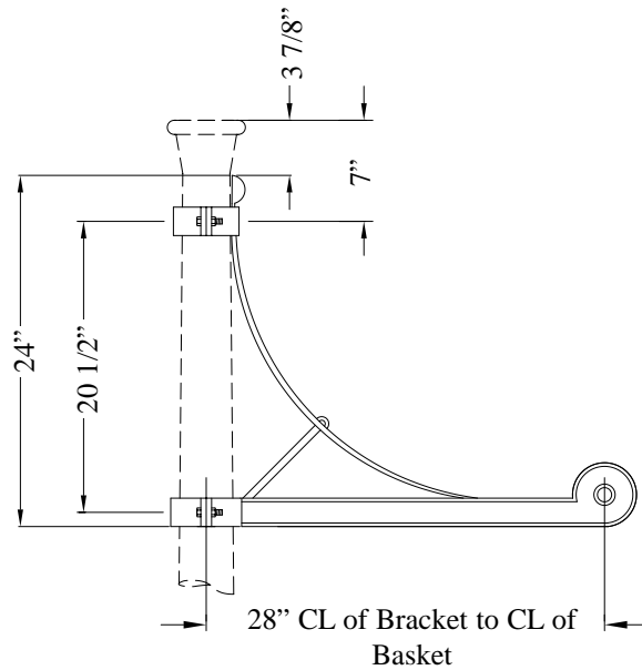
1 AARWSH -BK-CM-CB 1 Cast Aluminum Arm Washington - Flower Pot Bracket - Clamp Mount - Classic Black Finish
