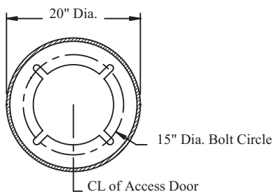
Northampton Lighted Bollard BDNRT-20-3.81-LT
