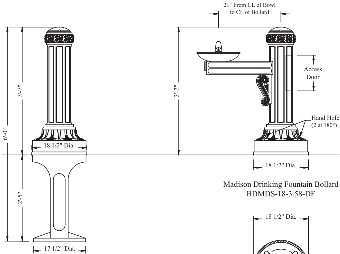
Madison Direct Burial Bollard BDMDS-18-3.58-DD
