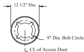
Northampton Lighted Bollard BDNRT-12-3.04-LT
