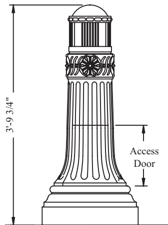
Northampton Lighted Bollard BDNRT-20-3.81-LT
