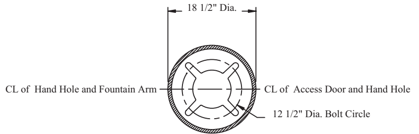
Madison Drinking Fountain Bollard BDMDS-18-3.58-DF
