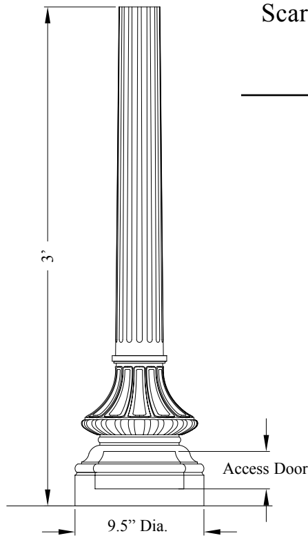
Scarsdale Parking Meter PSSCR-9-3
