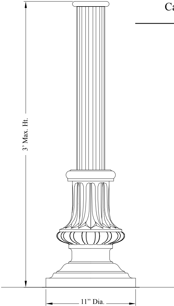
Washington Parking Meter Post PSWAH-11-3
